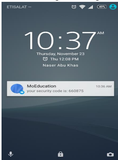
Figure 8: OTP SMS
